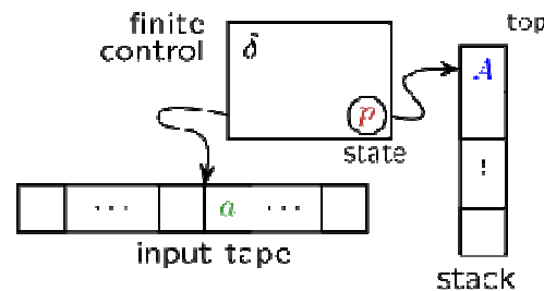
PDA
