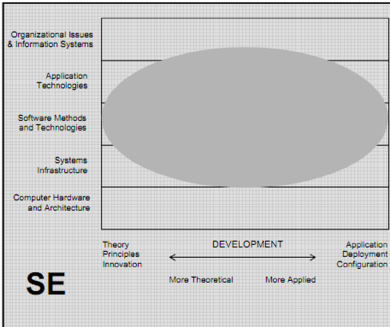
Figure 2.7. Software Engineering
