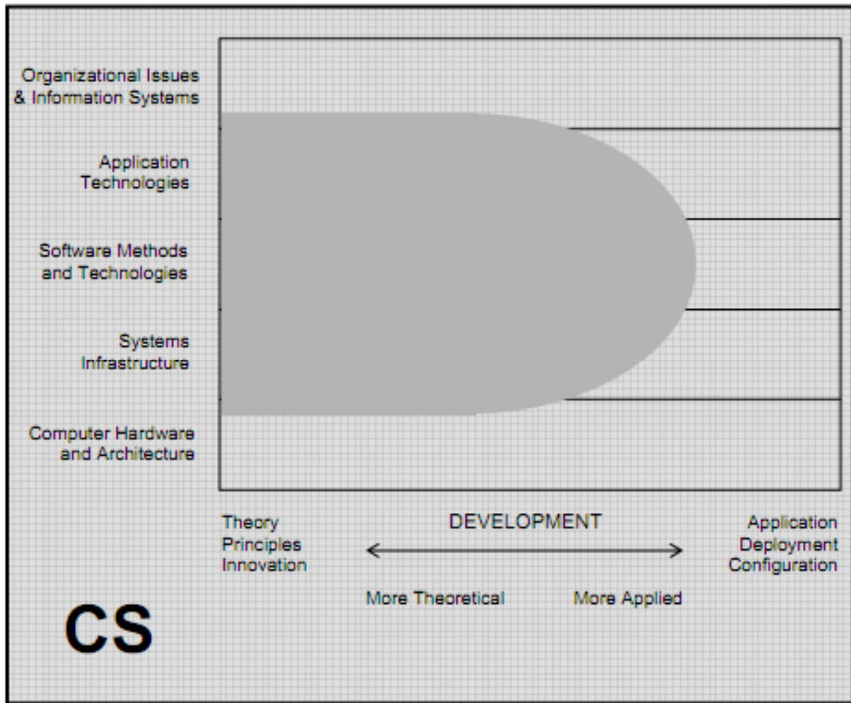
Figure 2.4. Computer Science
