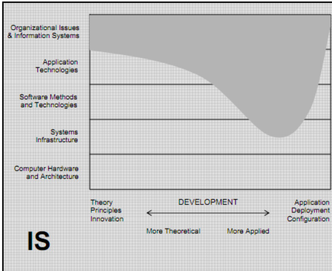
Figure 2.5. Information Systems
